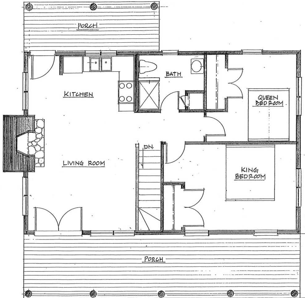
CABIN MAIN LEVEL PLAN
